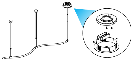
A suspension installation with surface mounted driver (with canopy)
